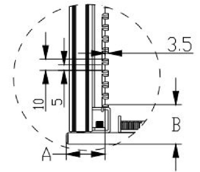
DETAIL D SCALE 2:1
